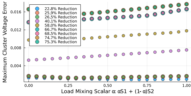
Fig. 5. Worst-case intra-cluster voltage errors for all iterate Kron-reduced versions of the meshed 200-node system (optimally reduced via nine iterations in Alg. 1). Reductions are given in terms of load bus reductions.
