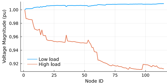
Fig. 3. The voltage profile resulting from two distinct net-load injections in the radial 115-node network. The red line represents a heavily loaded scenario, while the blue line represents a lightly loaded scenario with more solar PV injections.
